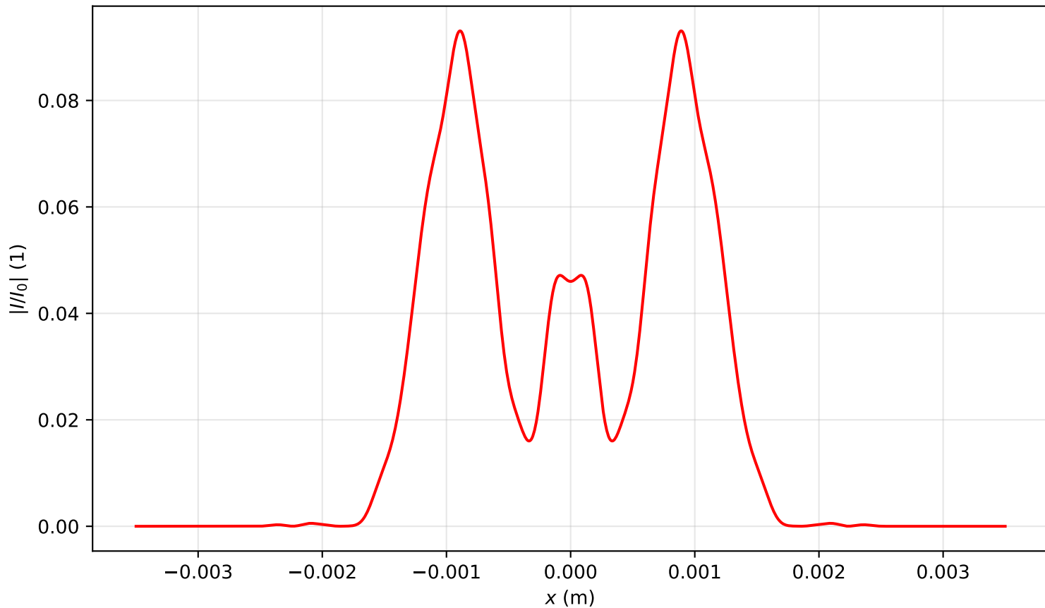
Intensity profile I(x, y = 0, z = 2.627)/I_0 , P_{in}=7.5P_{cr} , artificial time
